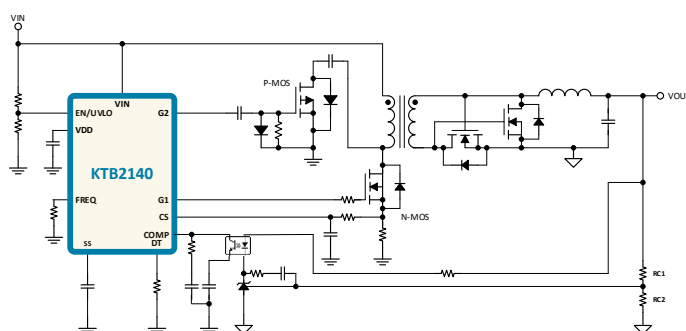
Active Clamp Current-Mode PWM Controller
