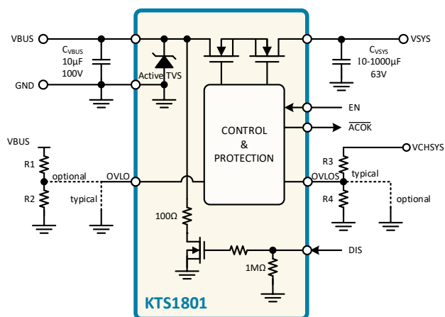
REPLACE W/ KTS1801 Block Diagram 48V/7A, ±180V Surge, Bi-Directional Load Switch with OVP, OCP, RBP, RCP, CL, SCP and POK Safe LDO
