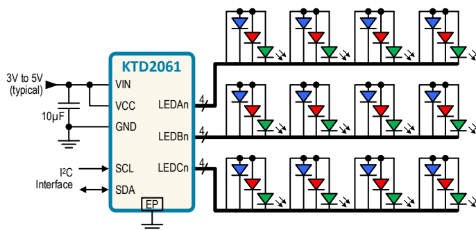
36-Channel RGB LED Driver with I 2 C Control
