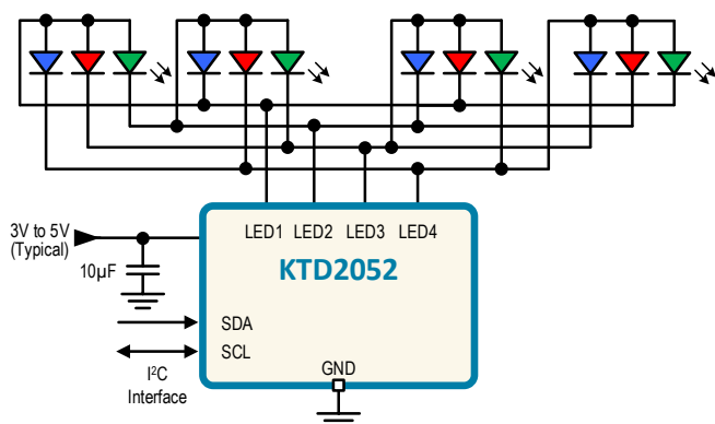
12-Channel RGB LED Driver with I 2 C Control
