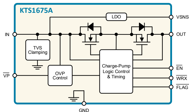
20V/5A, \pm 100V Surge, 13V/23.4V Fixed OVP with RBP & OTG
