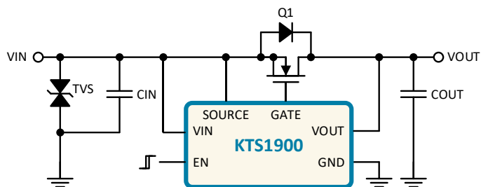
Ideal Diode and Load Switch Controller with Reverse Input Protection
