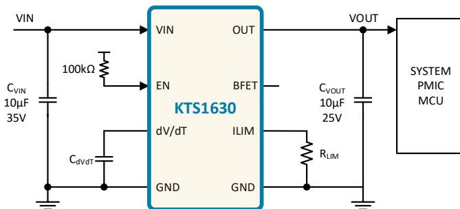
5V eFuse with Current Limit Control and Reverse Blocking FET Control
