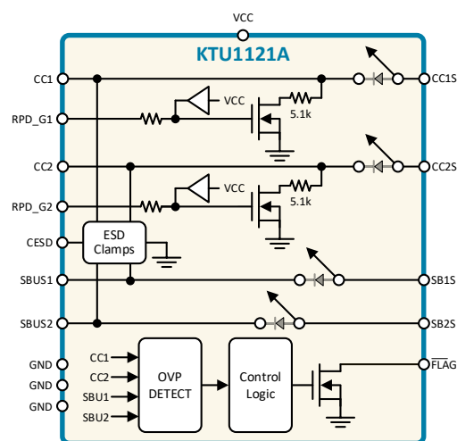
USB Type-C Port Protector for CC and SBU Pins
