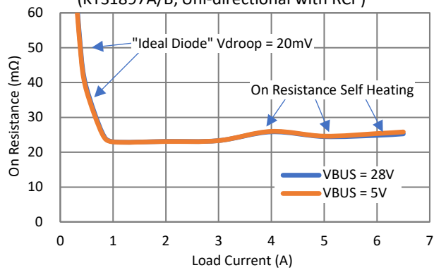
On Resistance Vs. Load Current (KTS1897A/B, Uni-directional with RCP)
