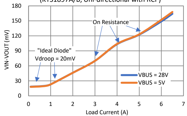
"Ideal Diode" Vdroop Vs. Load Current (KTS1897A/B, Uni-directional with RCP)
