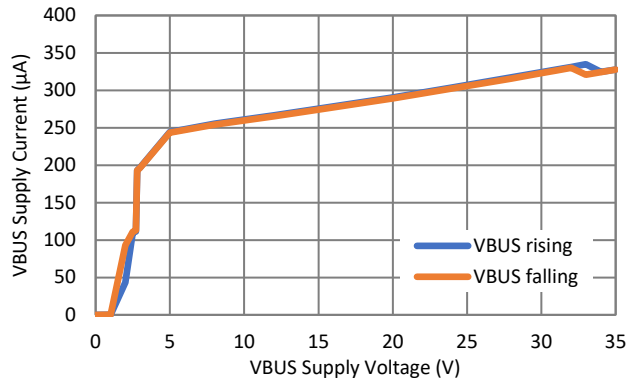
VBUS Supply Current Vs. Supply Voltage (No Load, EN = High)
