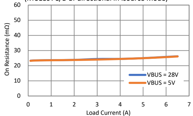
On Resistance Vs. Load Current (KTS1897C/D Bi-directional in Isource Mode)
