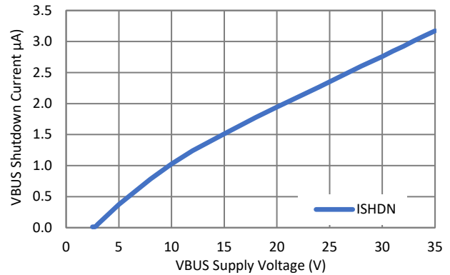
VBUS Supply Current Vs. Supply Voltage (No Load, EN = Low)
