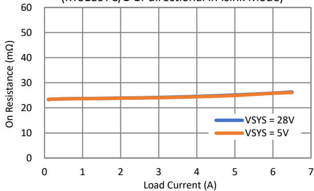
On Resistance Vs. Load Current (KTS1897C/D Bi-directional in Isink Mode)
