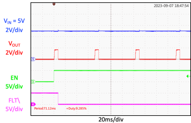
Over-Load Soft-Start & Auto-Retry Response ( FON = low , C_{OUT} = 10\mu F , R_{LOAD} = 1.5\Omega )
