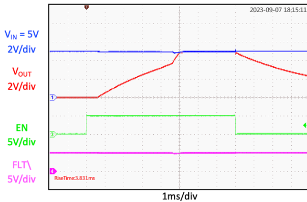
Heavy Load Soft-Start Response ( FON = low , C_{OUT} = 1000\mu F , R_{LOAD} = 6\Omega )
