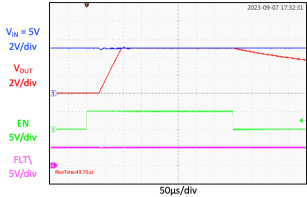
Fast On Enable, Soft-Start, Shutdown Response ( FON = high , R_{LOAD} = 100\Omega )
