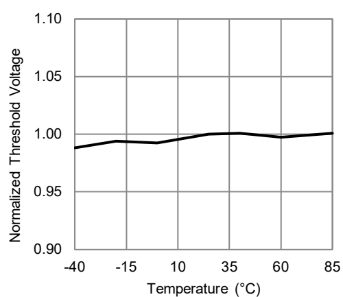
Normalized Adjustable OVLO Threshold vs. Temp.
