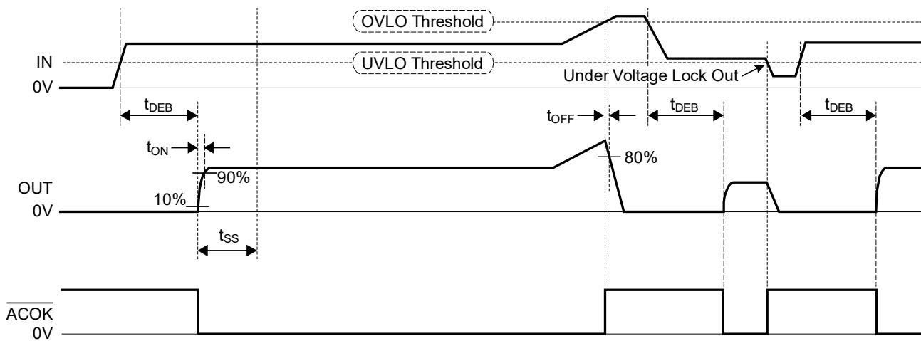
Figure 1. Timing Diagram
