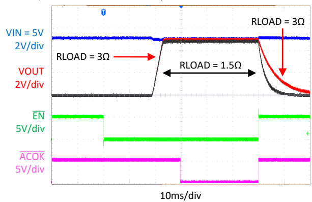
Heavy Load Soft-Start Response ( V_{OUT} = 5V , C_{IN} = 2000\mu F , KTS1673C/D I_{SOURCE} Mode)
