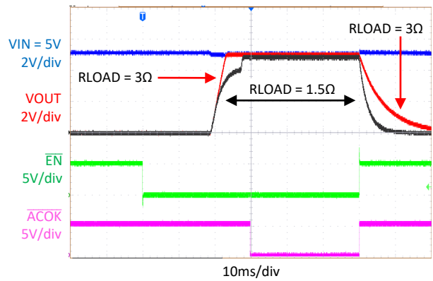
Heavy Load Soft-Start Response ( V_{IN} = 5V , C_{OUT} = 2000\mu F , KTS1673A/B/C/D I_{SINK} Mode)
