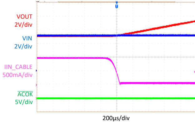
RCP Response KTS1673A/B Uni-directional with RCP (VIN = 5.1V, R_{CABLE} = 200m\Omega , Load = 5 \Omega , VOUT = 5V → 9V)
