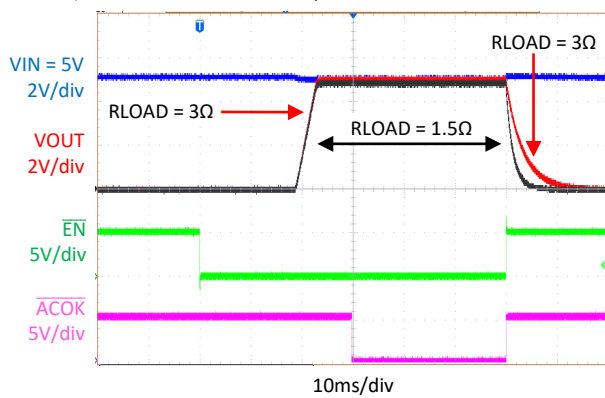
Heavy Load Soft-Start Response ( V_{OUT} = 5V , C_{IN} = 1000\mu F , KTS1673C/D I_{SOURCE} Mode)
