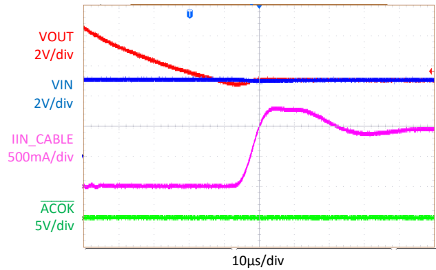
RCP Fast Recovery KTS1673A/B Uni-directional with RCP (VIN = 5.1V, R_{CABLE} = 200m\Omega , Load = 5 \Omega , VOUT = 9V → 5V)
