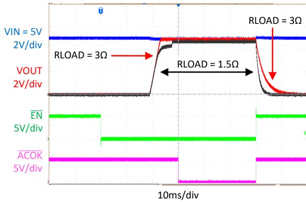
Heavy Load Soft-Start Response ( V_{IN} = 5V , C_{OUT} = 1000\mu F , KTS1673A/B/C/D I_{SINK} Mode)
