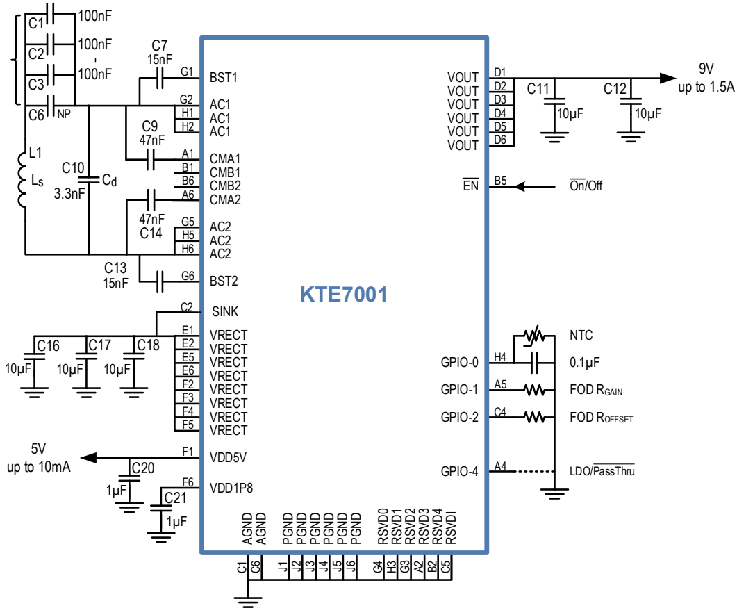
Figure 1. Detailed Application Schematic
