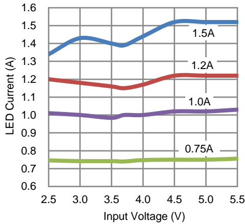
Torch LED Current vs. VIN (2MHz, 187.5mA per channel)
