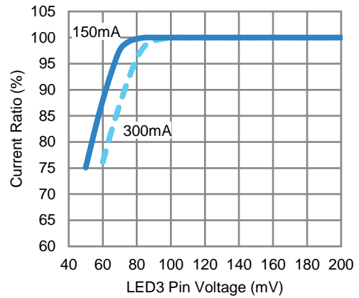
LED3 Pin Dropout Voltage
