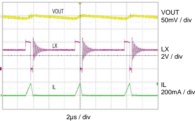
Switching waveform Global LED (9 LEDs at 1.5mA/channel, Skip mode)
