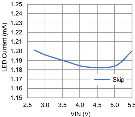
LED Current vs. VIN (Global ILED = 1.2mA)
