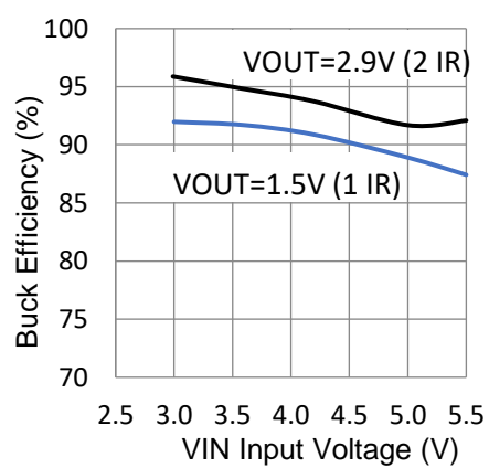
Buck Efficiency v. VIN (9 channels at 20mA, Skip-mode)
