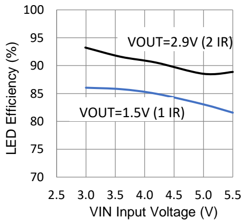
LED Efficiency vs. VIN (9 channels at 20mA, Skip-mode)
