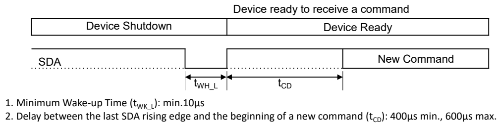
Figure 6. Wake-up from Shutdown Mode
