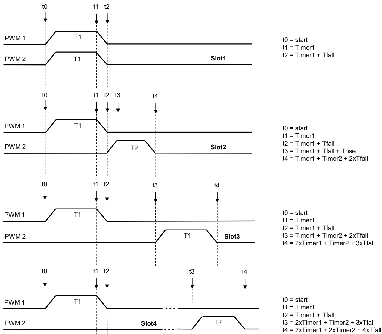
Figure 3. Timer Slot Timing Diagram
