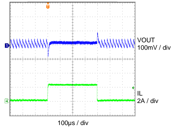
Load Transient (0A-4.5A, Auto-Skip Mode)
