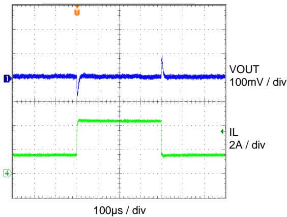
Load Transient (1.5A-4.5A, Auto-Skip Mode)
