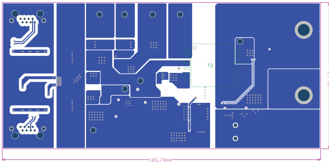
Bottom Layer Routing
