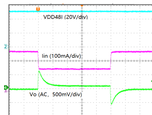
2ms / div
