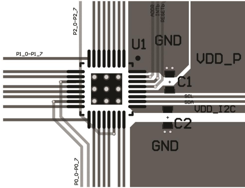
Figure 10. Recommended Layouts for TQFN55-32
