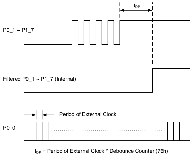
Figure 9. Debounce Timing
