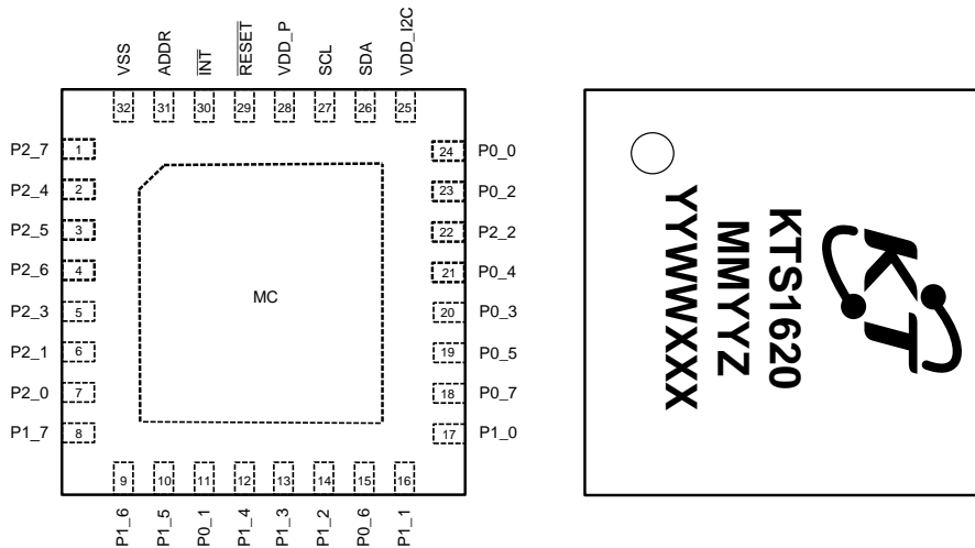
32-Lead 5mm x 5mm x 0.75mm TQFN55-32 Package
