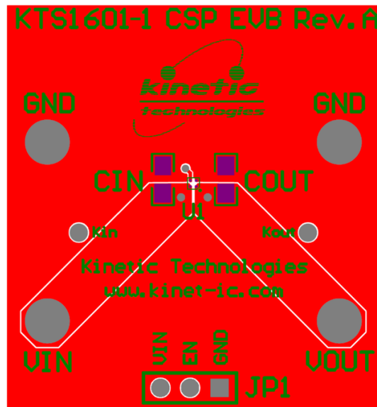
Figure 2. KTS1601-1 Evaluation Board Layout (TOP Layer)
