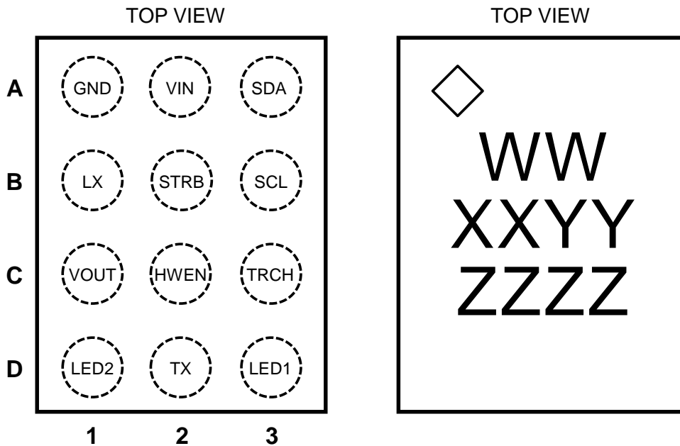
12-Bump 1.42mm x 1.66mm x 0.62mm WLCSP Package
