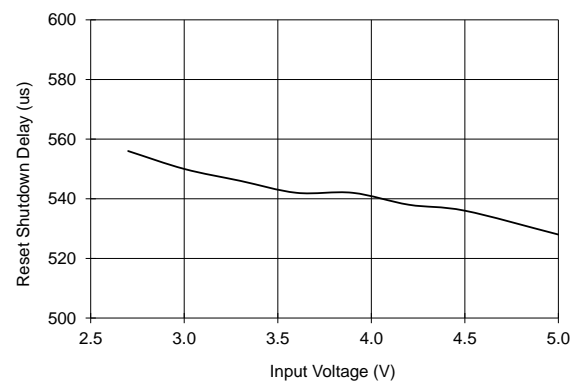
Reset Shutdown Delay vs. Input Voltage
