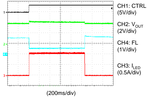
Flash Timeout Operation (1049ms setting)
