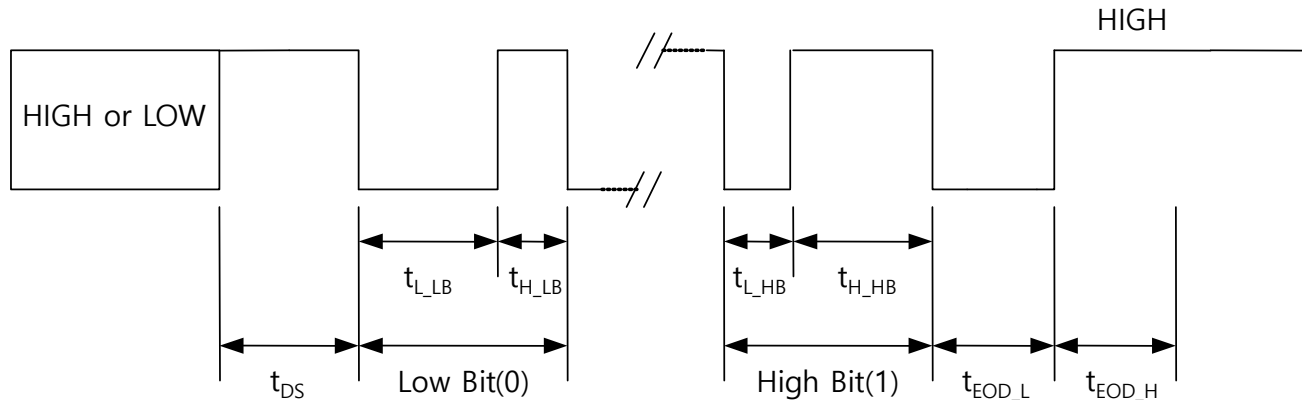
Figure 5. ExpressWire Interface – Bit Coding Time
