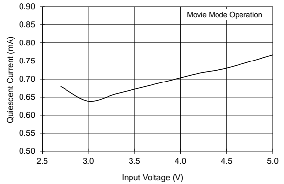
Movie-mode Operating Current
