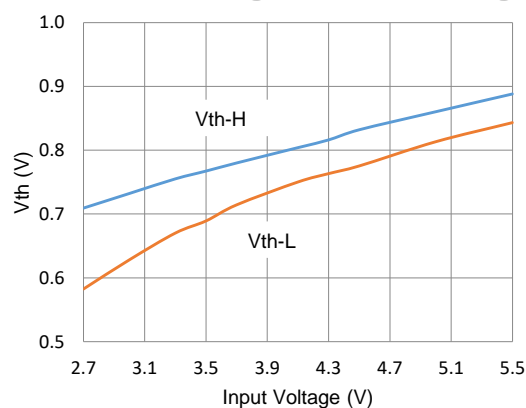
ENP / ENN Logic Threshold Voltage
