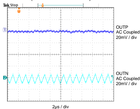
Steady-state Operation ( I_{POS} = -I_{NEG} = 40mA )
